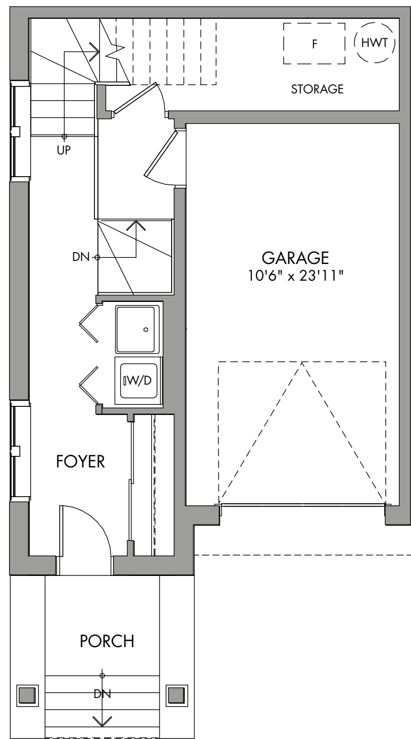
LEVEL 1
