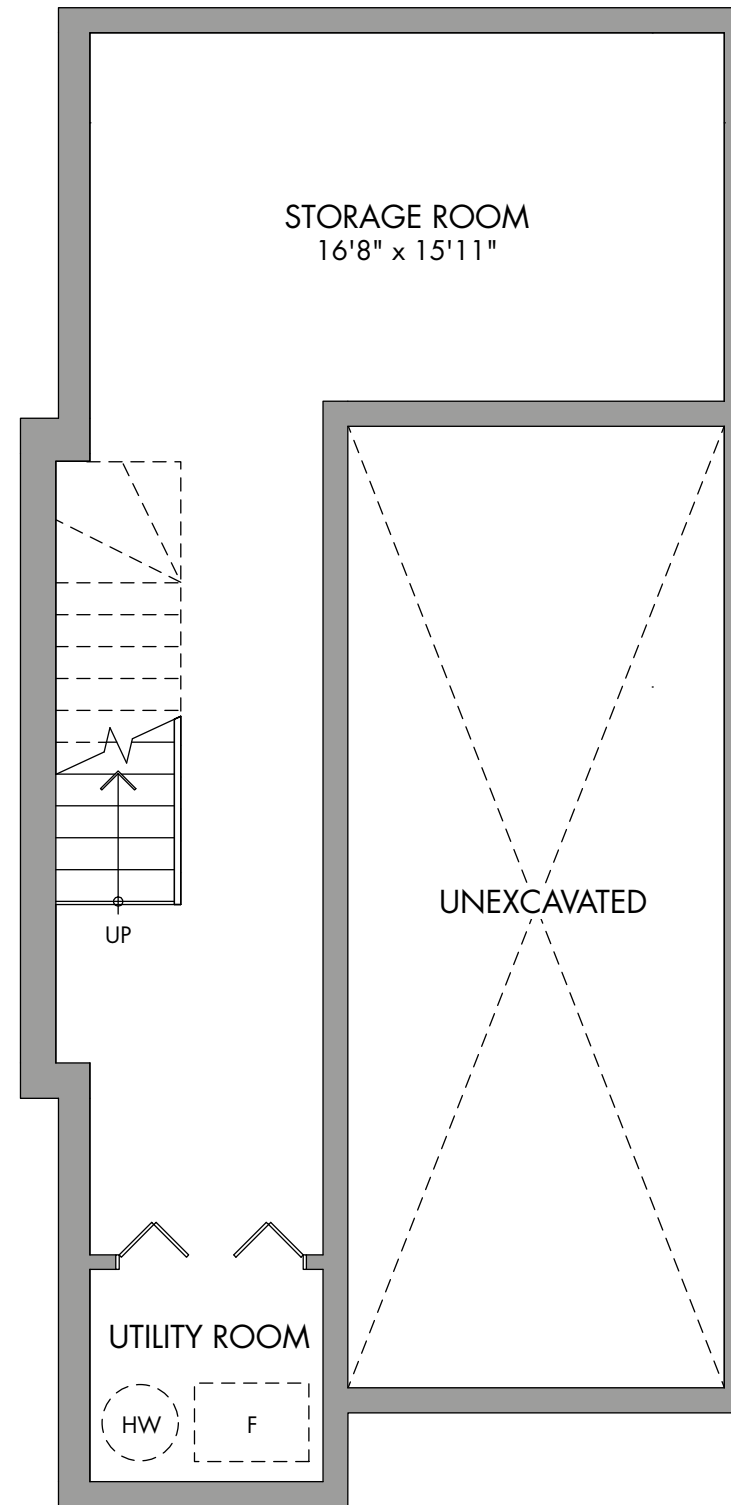
BASEMENT
