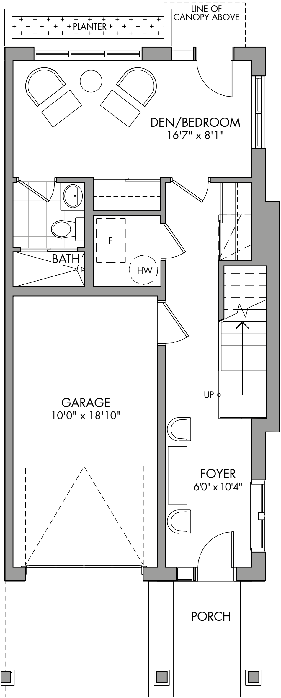
LEVEL 1
