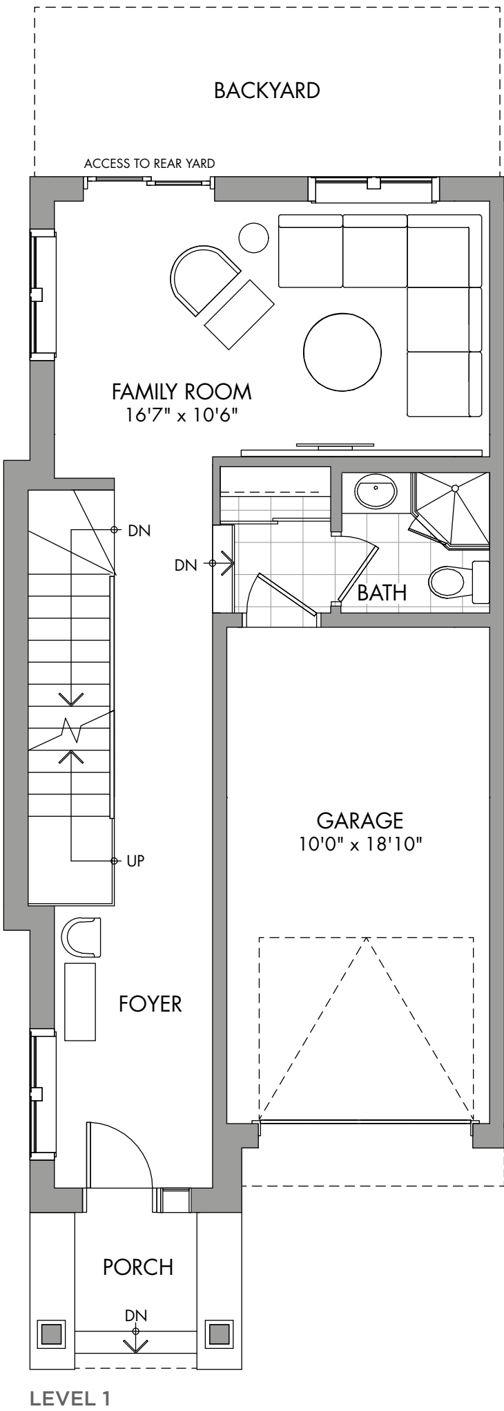
LEVEL 1
