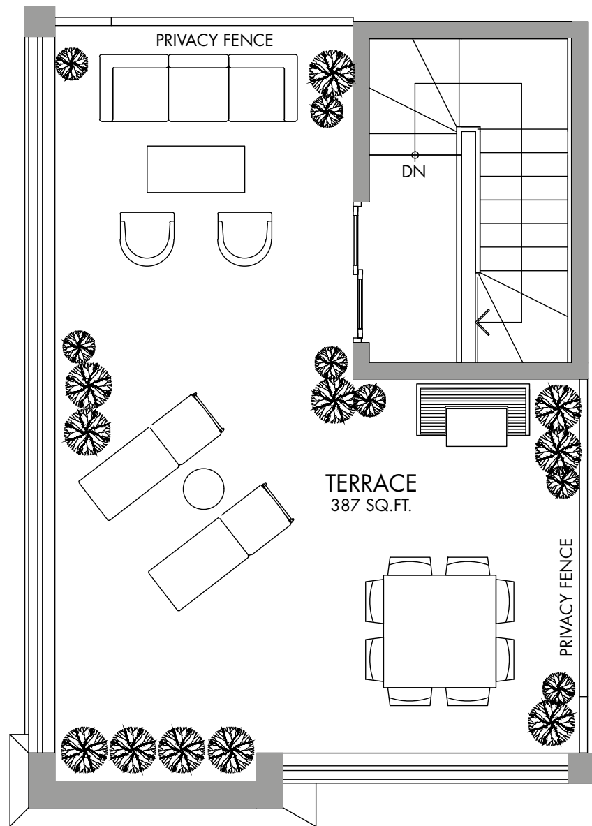
ROOFTOP TERRACE
