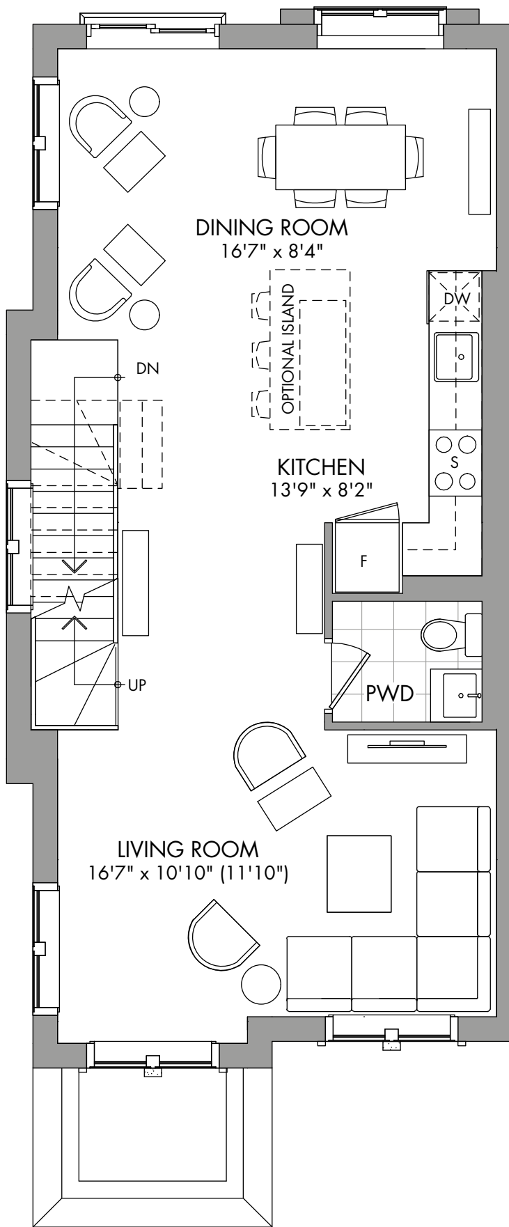
LEVEL 2
