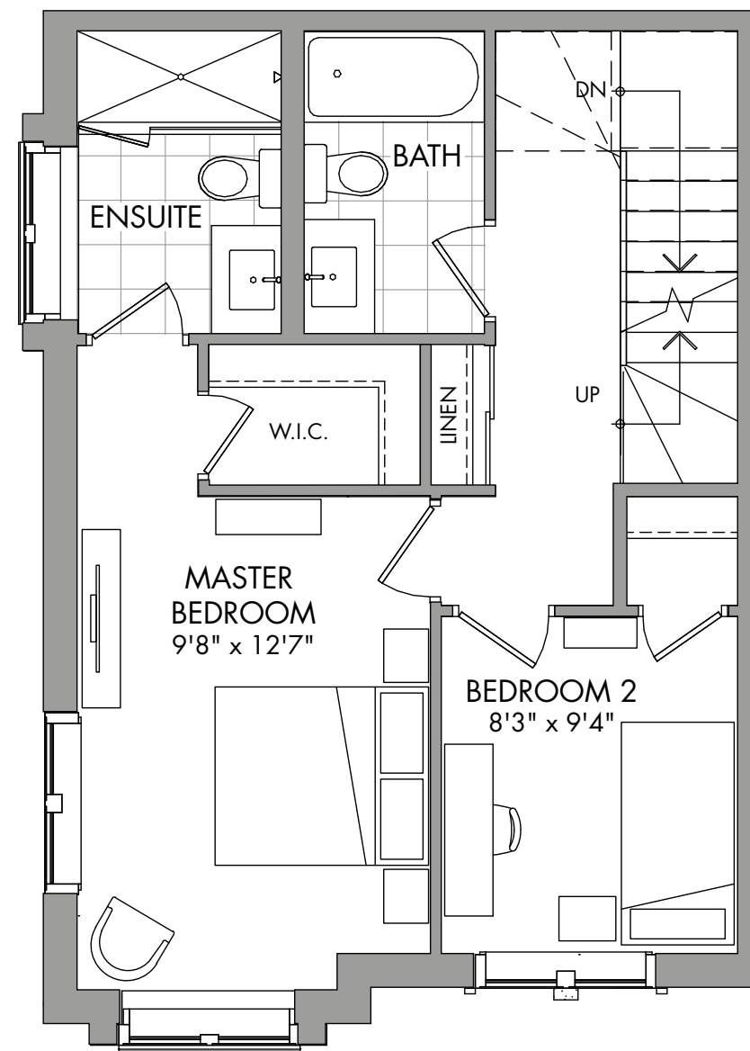
LEVEL 3
