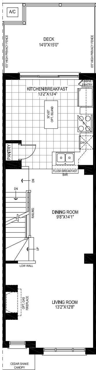
Main Floor
