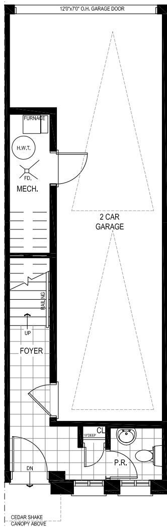
Ground Floor
